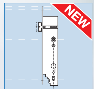
Motor lock 1956/1959 with integral electronics
